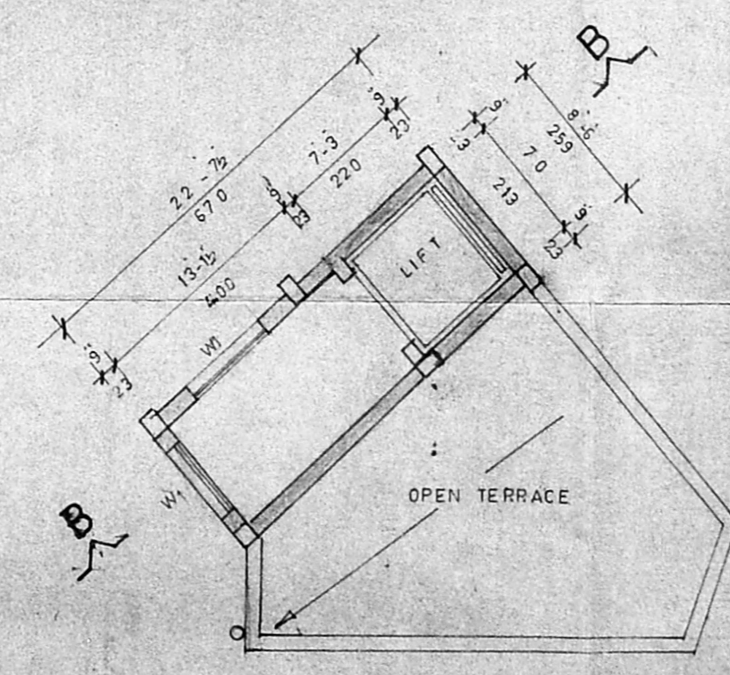
LIFT ROOM PLAN
