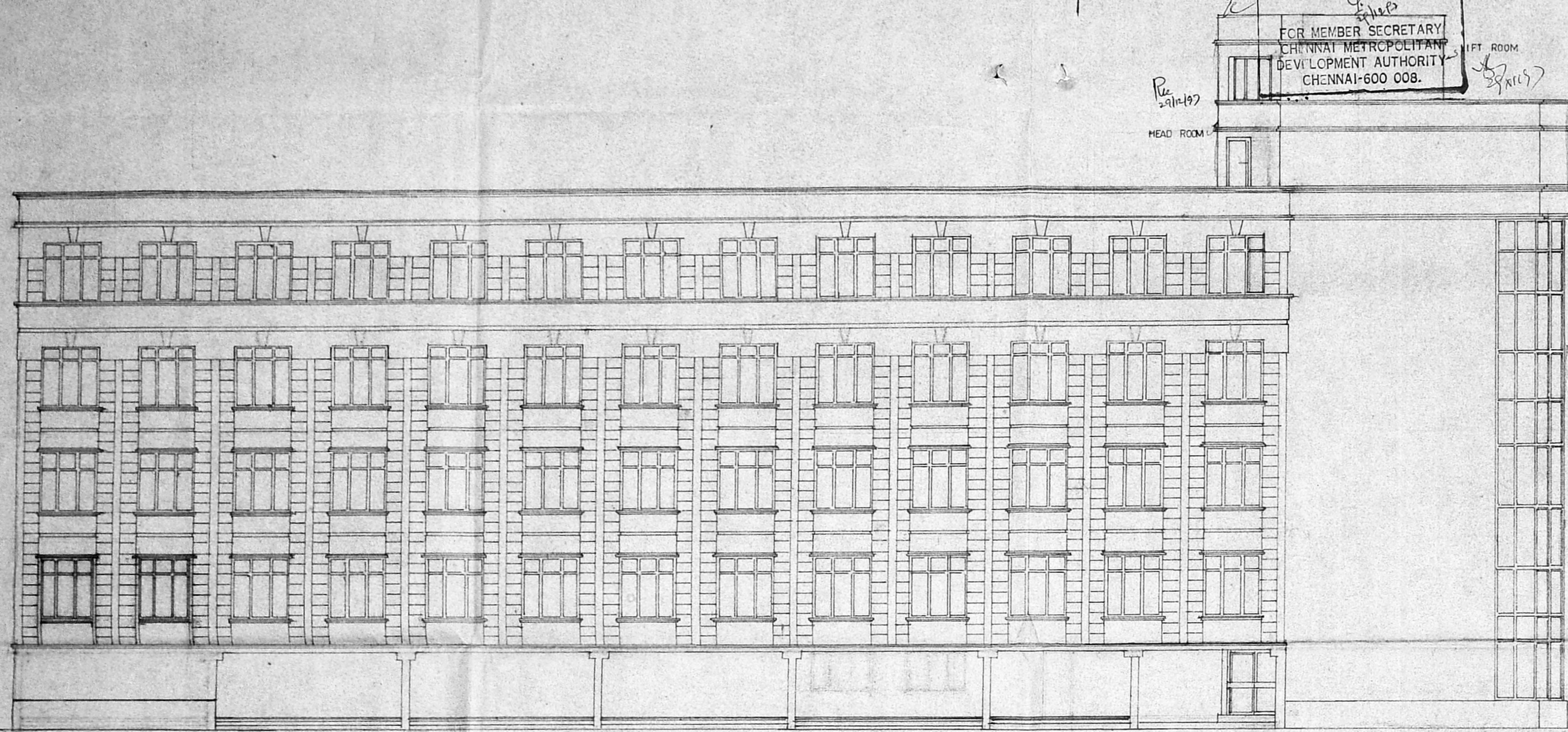
EASTERN SIDE ELEVATION
