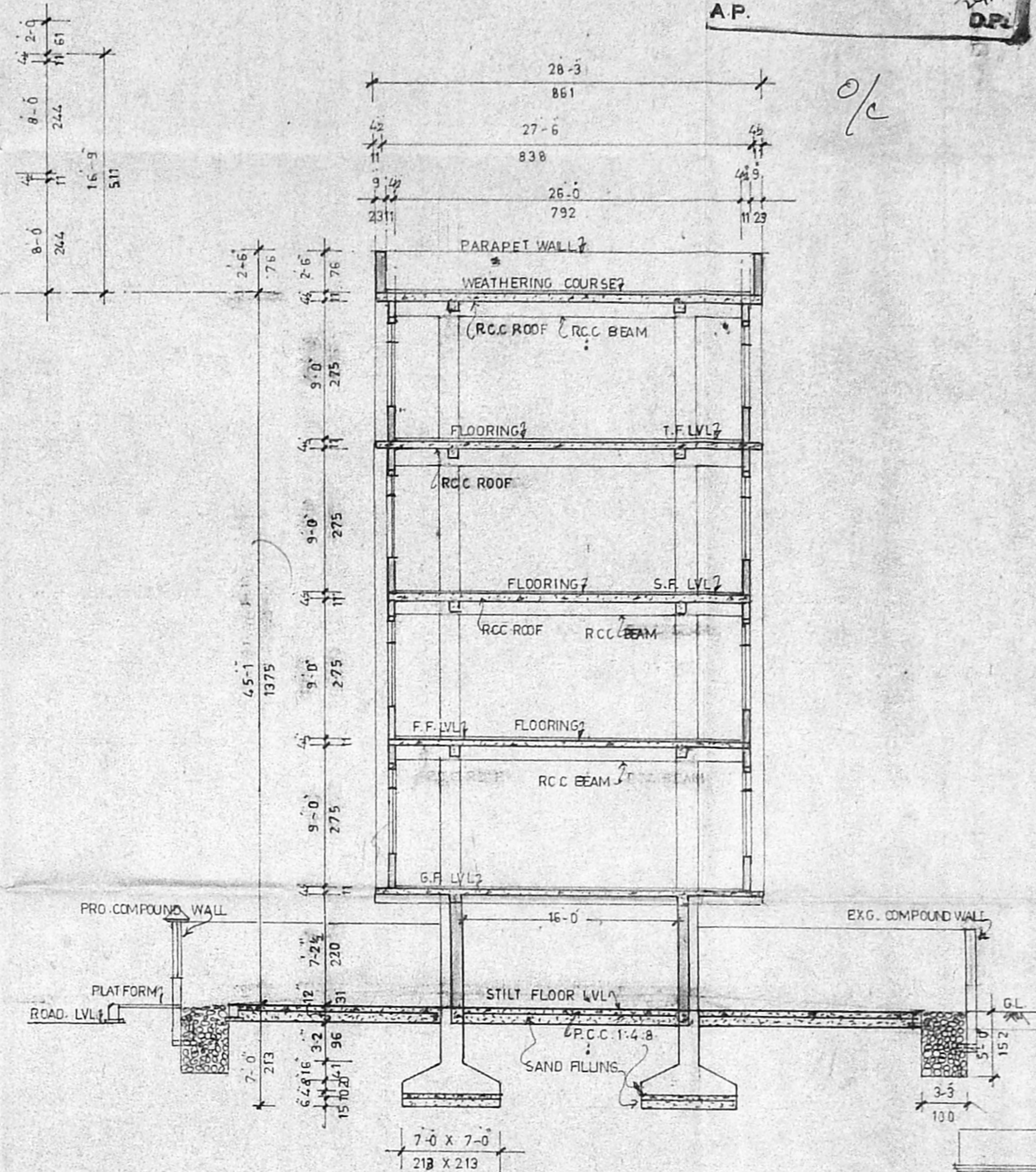
SECTION - AA
