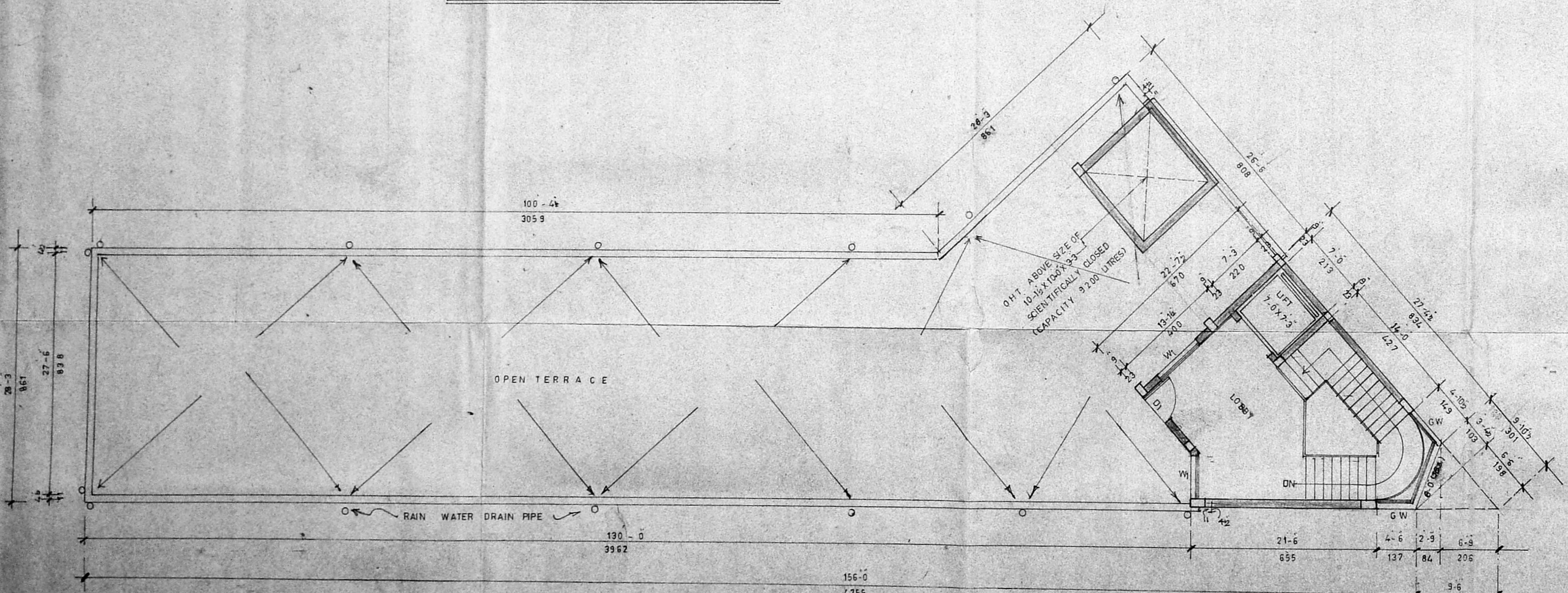
TERRACE PLAN
